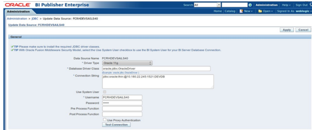
Figure 11–8 Data Source
