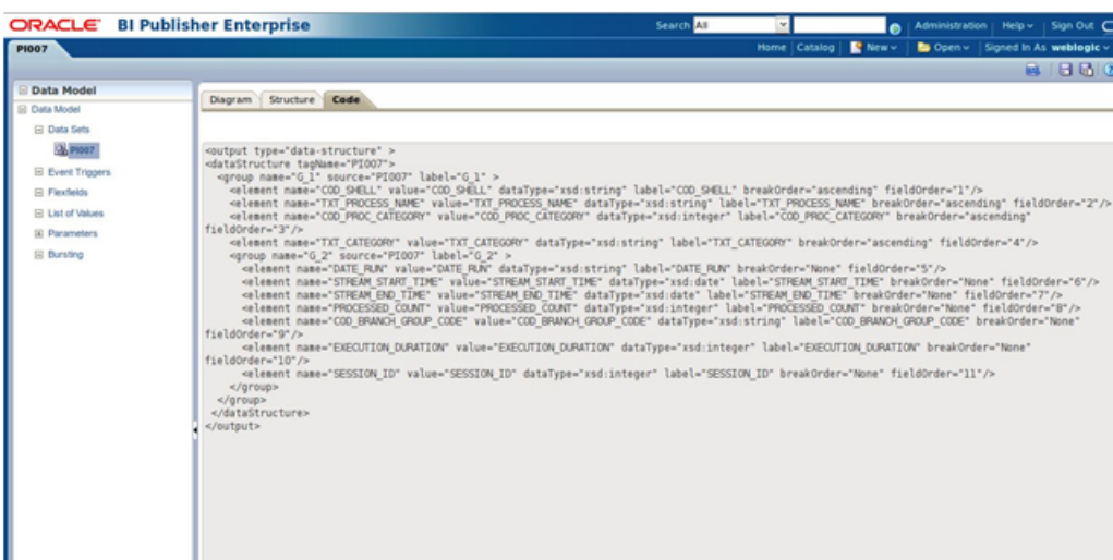
Figure 11–13 XML Code
